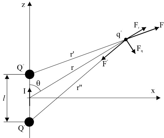
Figure 1: HERTZ Dipol
